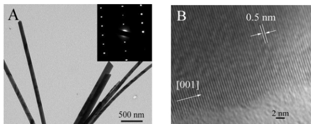
Fig. 3 (A) TEM image of as-prepared Se nanowires, the inset shows the SAED pattern of a single nanowire; (B) representative HRTEM image of as-prepared Se nanowires; the [001] direction is coincident with the nanowire axis.
