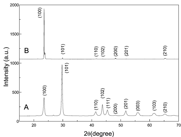
Fig. 2 XRD patterns of commercial selenium powder (A) and as-prepared selenium single-crystal nanowires (B).
