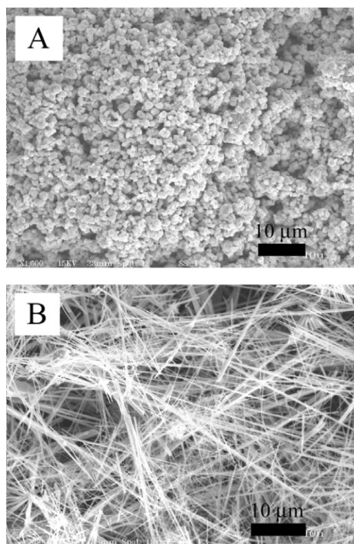
Fig. 1 SEM images of commercial poly-crystalline selenium powder (A) and as-prepared, single-crystal selenium nanowires (B); the scale bar is 10 \mu\text{m} .
